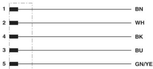
Contact assignment of the M12 plug
